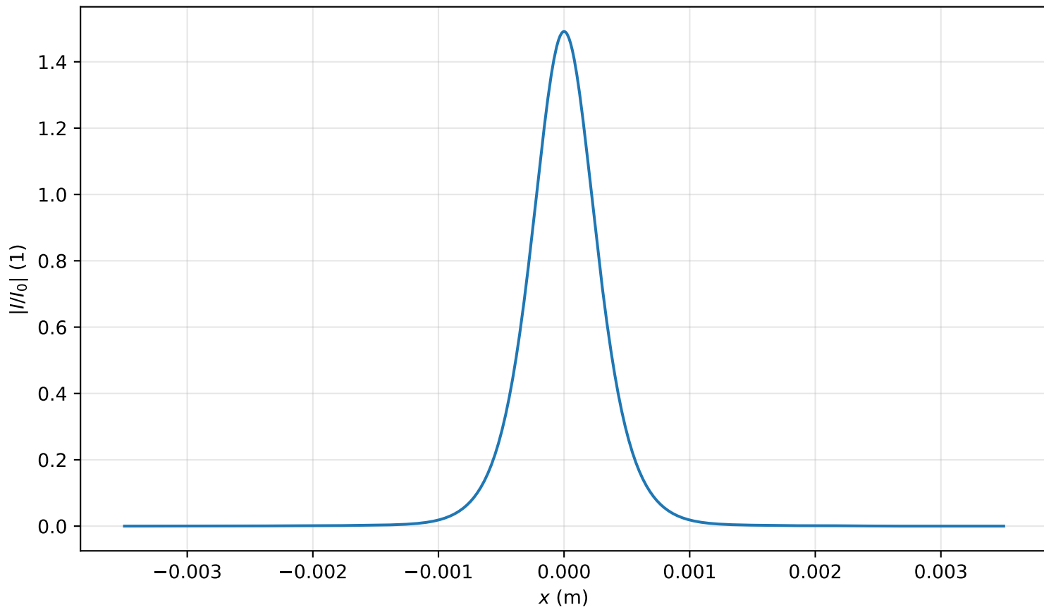
Intensity profile I(x, y = 0, z = 3.503m)/I_0 , P_{in}=0.9P_{cr} , artificial time
